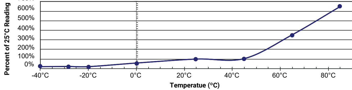
LEAKAGE CURRENT VS. TEMPERATURE
