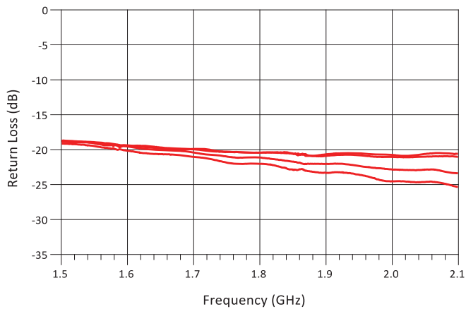
Return Loss
