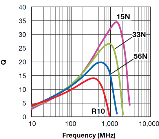
0402 Q VS Frequency
