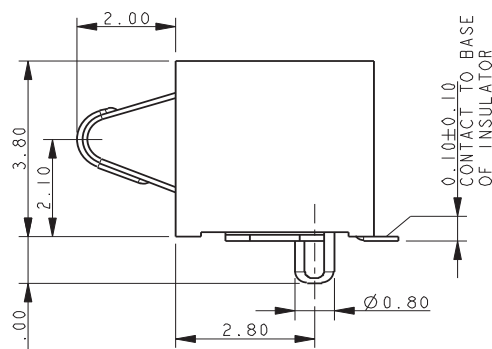
UNDEFLECTED CONTACT
