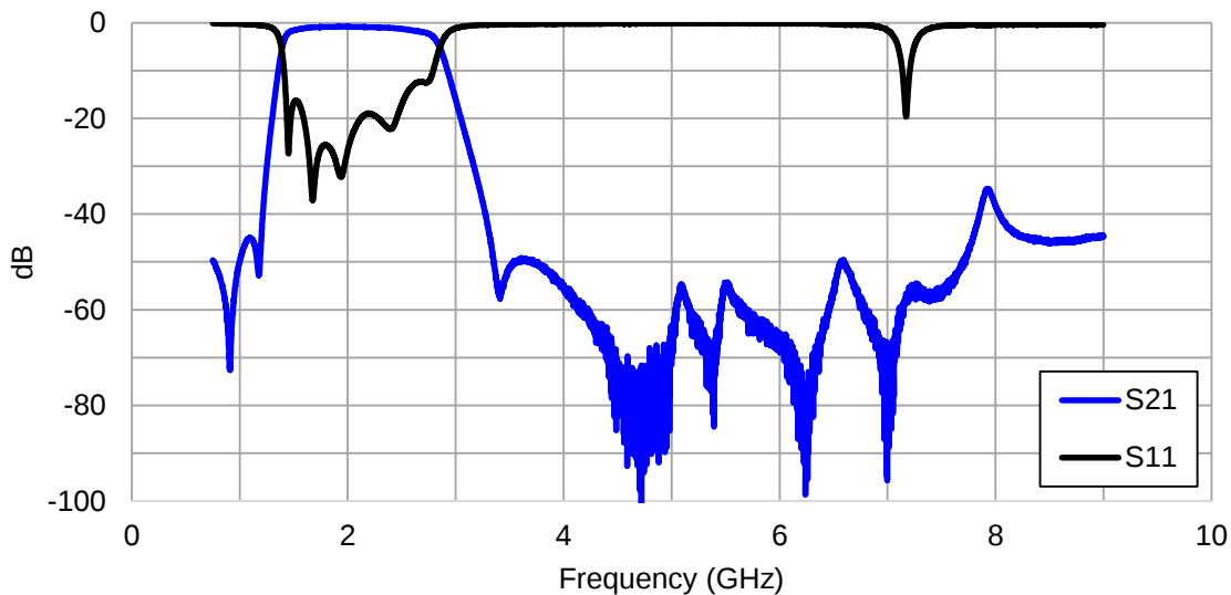
Typical Frequency Response
