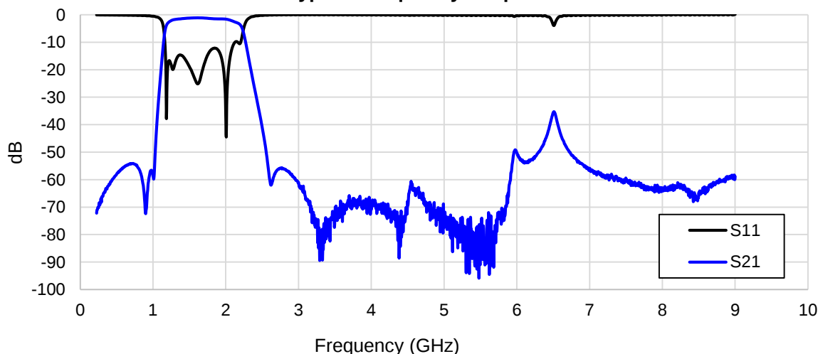
Typical Frequency Response
