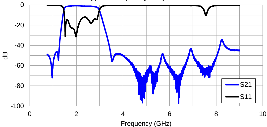
Typical Frequency Response
