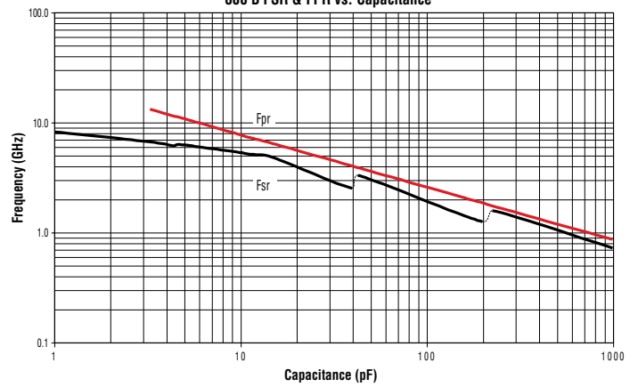
800 B FSR & FPR vs. Capacitance
