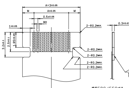
RECOMMENDED FPC/FFC
