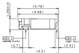
SECT. X-X
