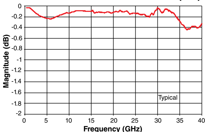
ATC 506WLSN10R7 Insertion Loss (S21)
