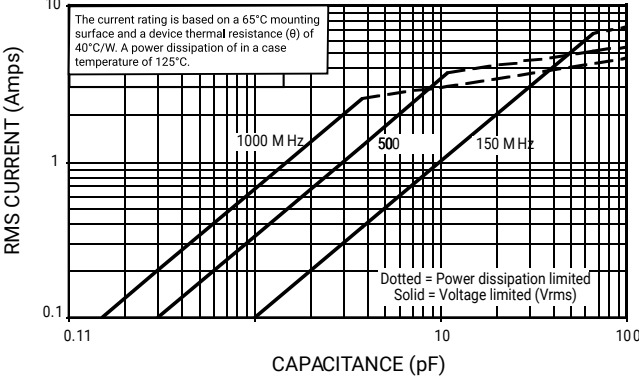
CURRENT RATING VS. CAPACITANCE SERIES 100, CASE A
