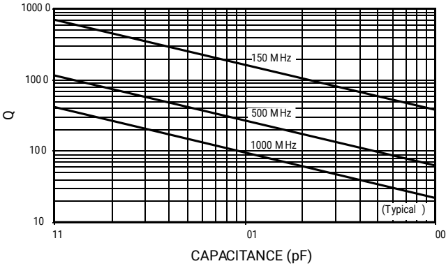
Q VS. CAPACITANCE SERIES 100, CASE A
