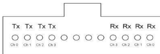
Figure 2 Optical Lane Assignment (front view of MPO receptacle)
