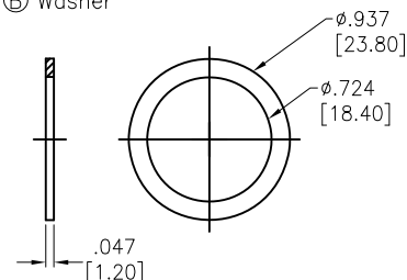
Ⓑ Washer
