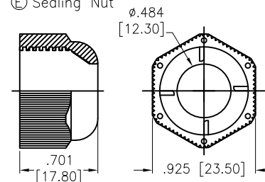
Ⓔ Sealing Nut
