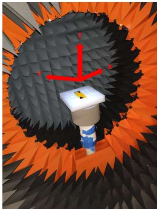
Chamber Set-up
