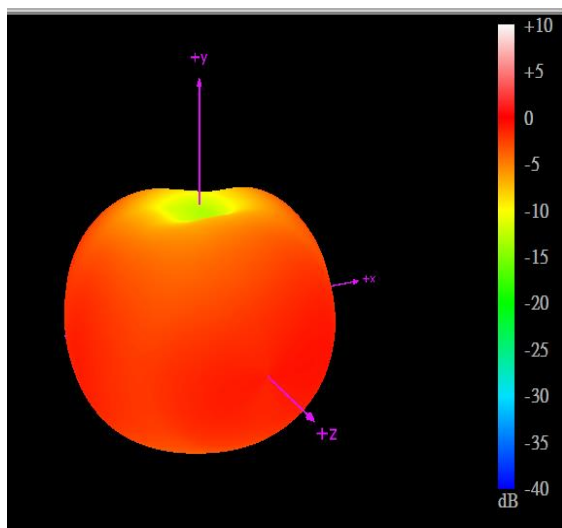
824MHz
