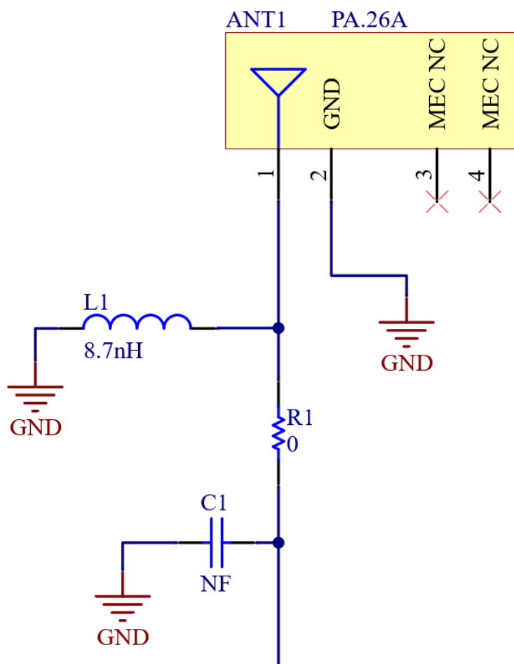
Matching Components
