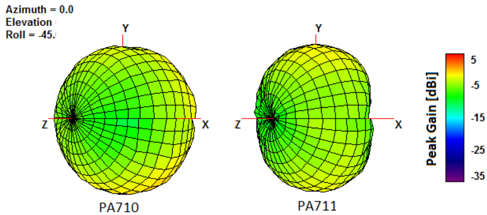
Figure 10. 3D Radiation Pattern at 700MHz of the PA.710 and PA.711 antennas
