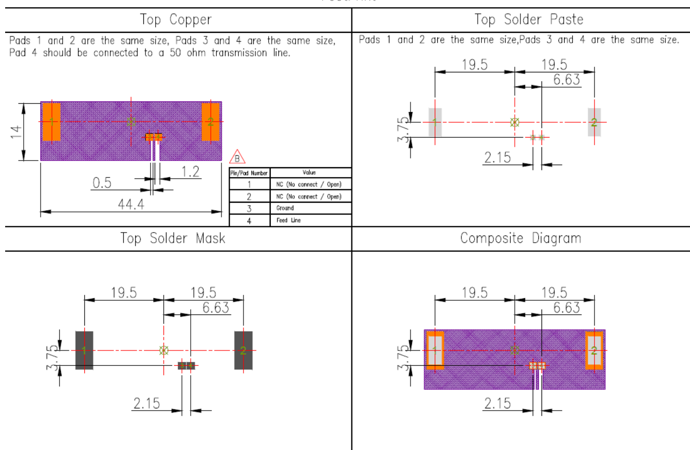
FootPrint
