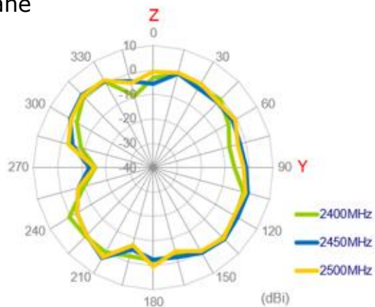
YZ Plane
