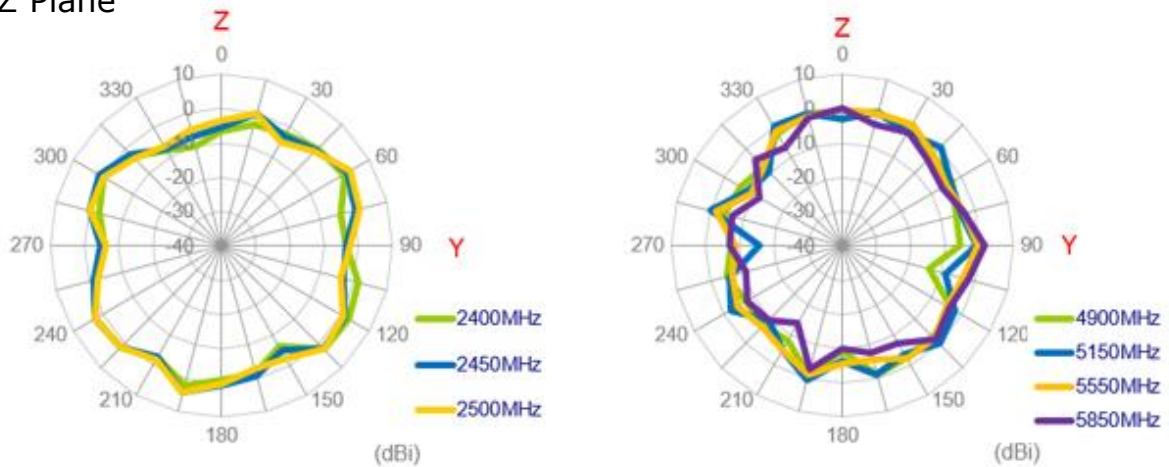
YZ Plane
