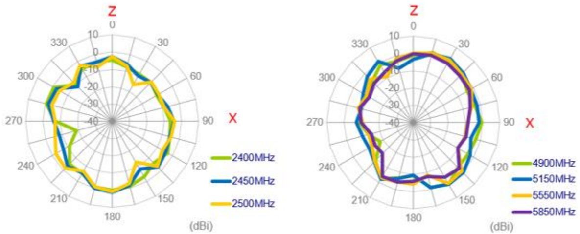
XZ Plane
