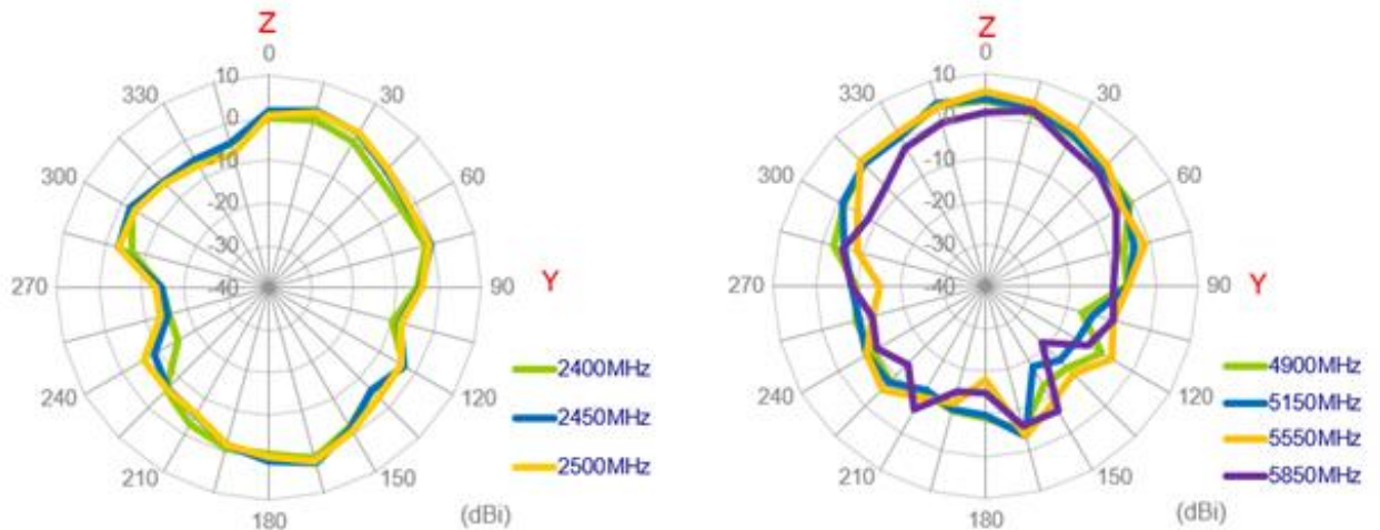
YZ Plane
