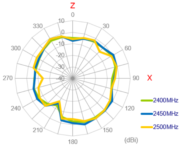
XZ Plane
