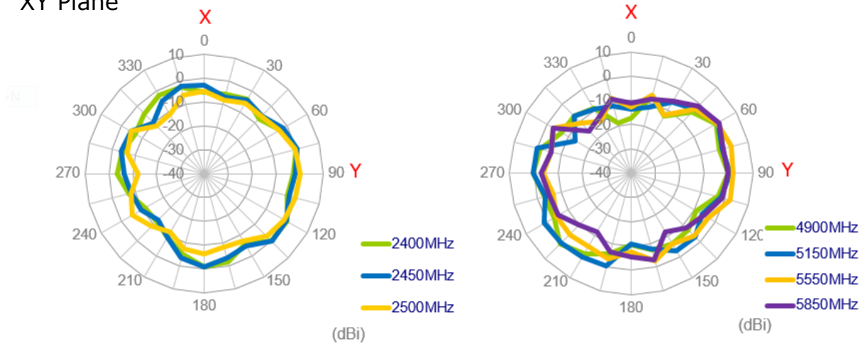
XY Plane
