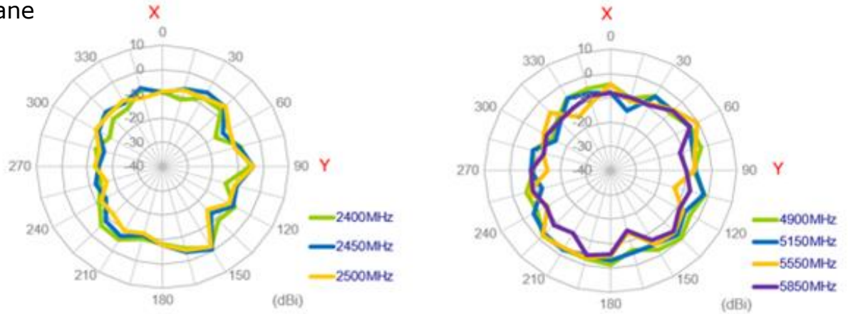
XZ Plane
