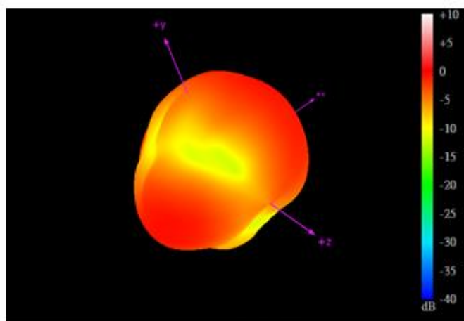
1575.42MHz
