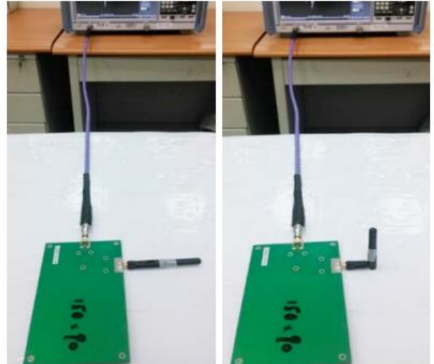
Antenna straight
