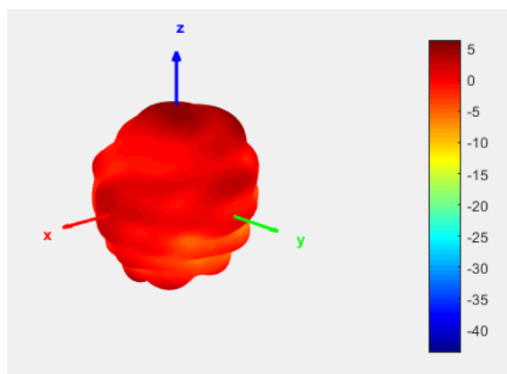
Radiation Pattern at 7.5GHz
