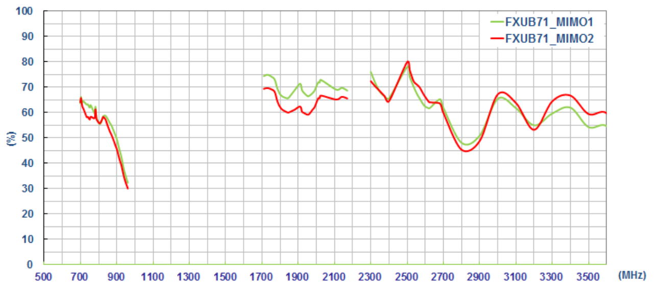
Figure3. Efficiency with 150 mm cable length and on the 2mm ABS of FXUB71
