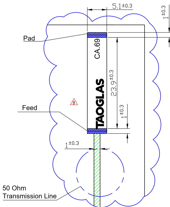
FR4 0.8t PCB Foot Print
