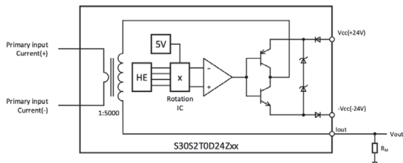
Figure 3 : Block diagram
