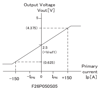
Figure 1 : Linearity curve (Internal reference voltage)
