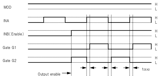
Timing chart of Half bridge mode
