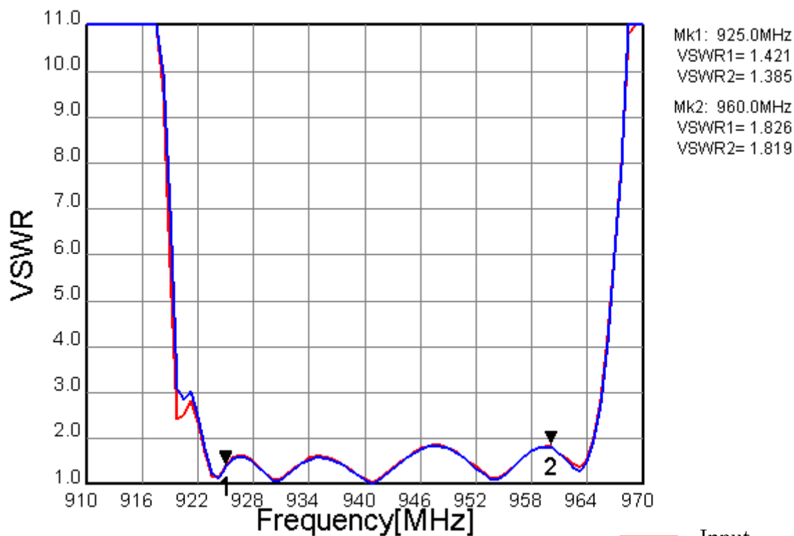
Fig.2 VSWR
