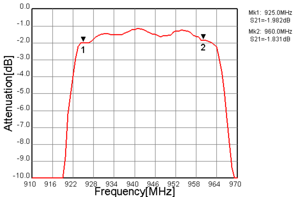
Fig.3 In-band Characteristics
