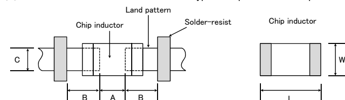
Recommended land dimensions for reflow-soldering (Unit: mm)
