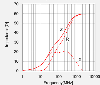
FB MJ2125HM330-TV
