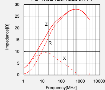
FB MJ2125HS250NTV
