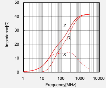
FB MJ1608HM230NTW
