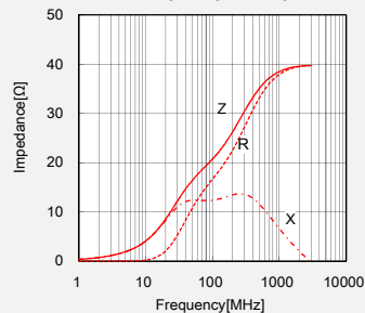
FB MJ2125HM210NTV
