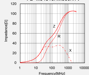
FB MJ4516HM560NTV
