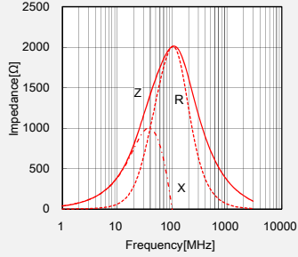
FB MH3225HM202NTV
