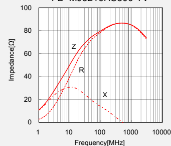
FB MJ3216HS800-TV
