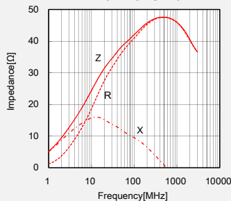
FB MJ2125HS420-TV
