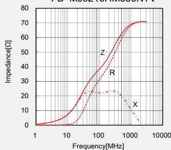
FB MJ3216HM380NTV
