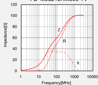
FB MJ3216HM600-TV
