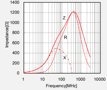
FB MH4516HM851NTV
