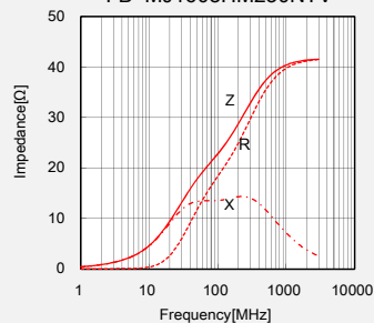
FB MJ1608HM230NTV
