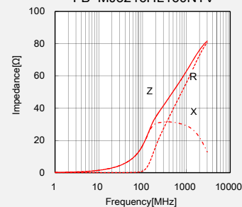
FB MJ3216HL160NTV
