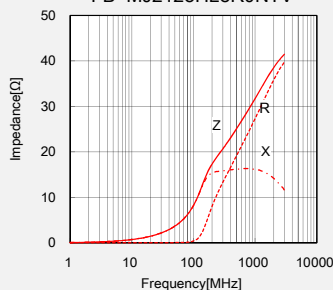
FB MJ2125HL8R0NTV
