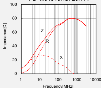
FB MJ4516HS720NTV
