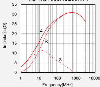
FB MJ1608HS280NTV
