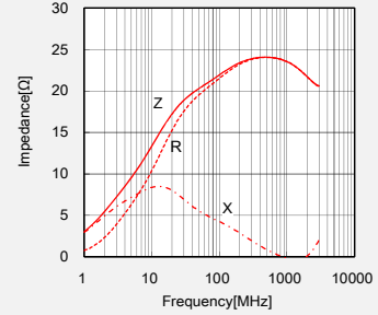
FB MJ1608HS220NTW
