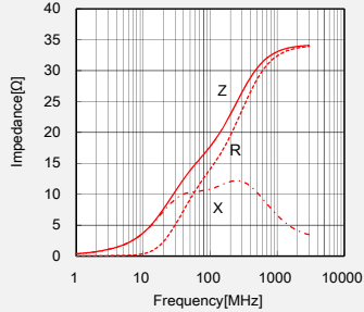
FB MJ1608HM180NTW
