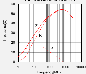
FB MJ3216HS480NTV
