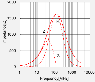
FB MH4525HM162NTV
