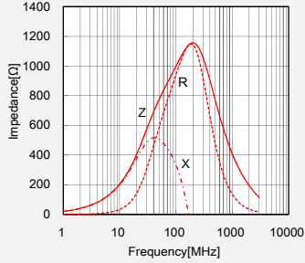
FB MH4525HM102NTV
