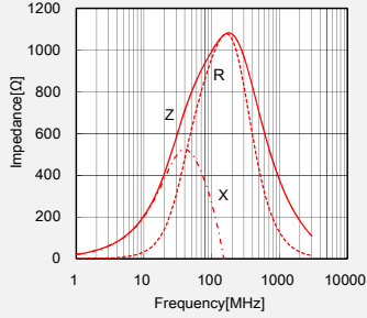
FB MH3225HM102NTV
