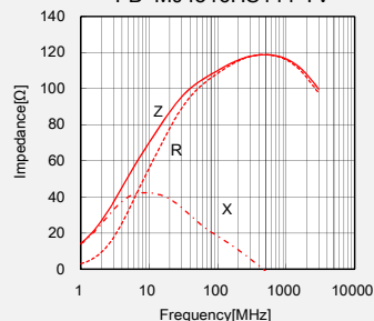
FB MJ4516HS111-TV
