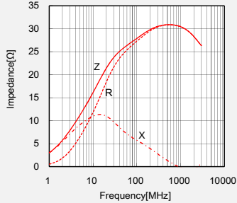
FB MJ1608HS280NTW
