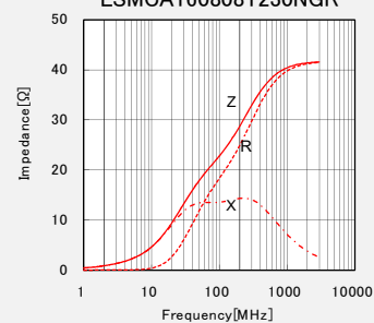
LSMCA160808T230NGR
