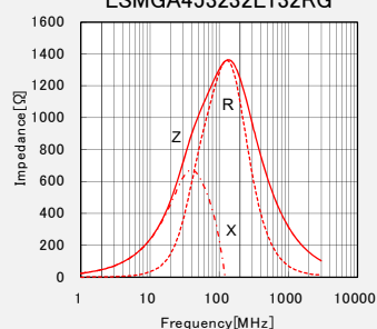
LSMGA453232L132RG
