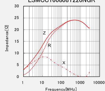
LSMCC160808T220NGR
