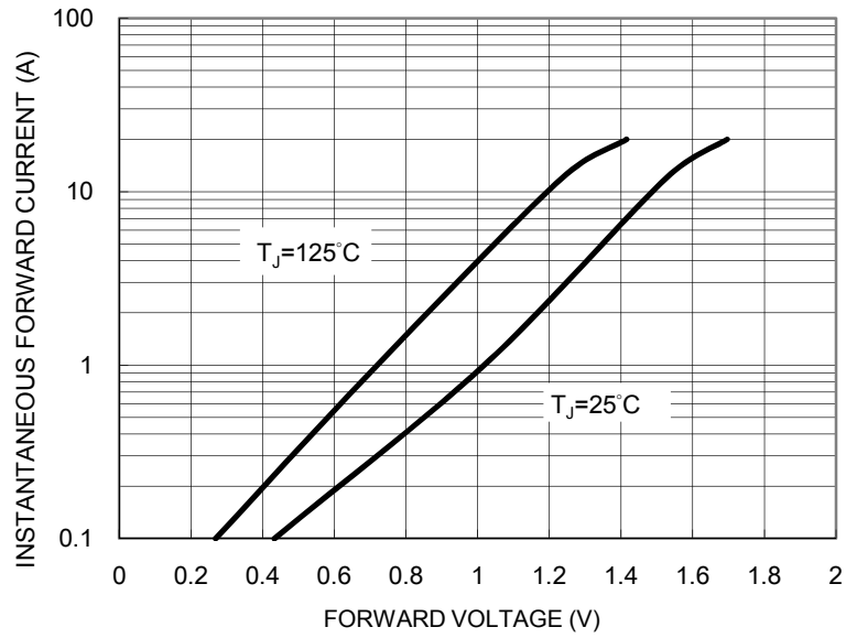
FIG. 4 TYPICAL FORWARD CHARACTERISRICS
