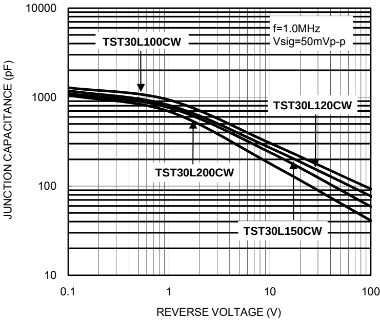
FIG. 10 TYPICAL JUNCTION CAPTIANCE
