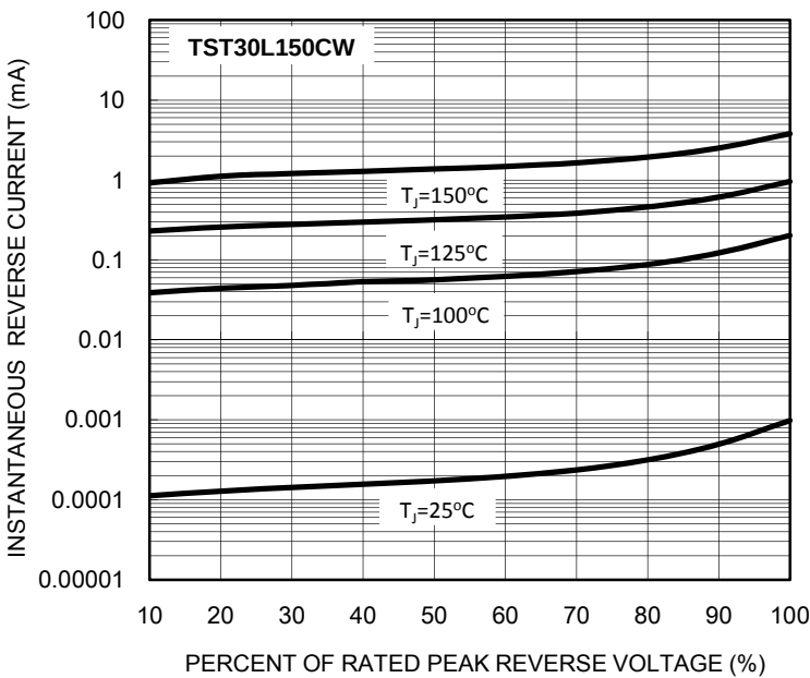
FIG. 8 TYPICAL REVERSE CHARACTERISTICS
