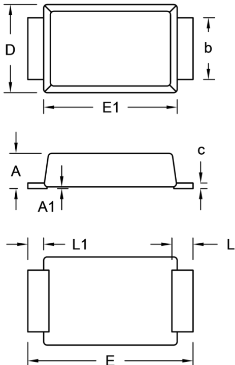
SOD-128
