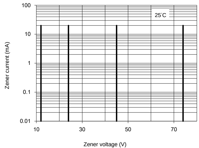
Fig.6 Zener breakdown characteristics
