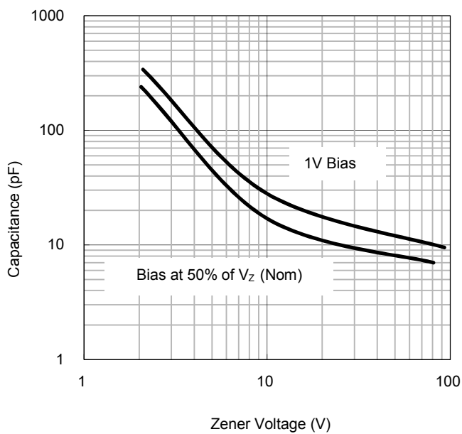
Fig. 3 Typical Capacitance
