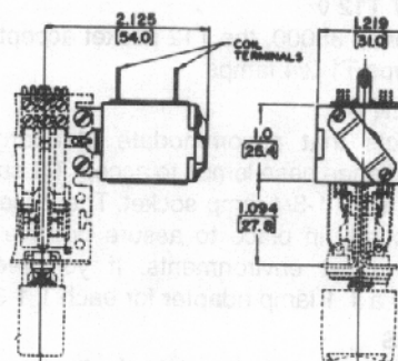
TYPICAL MOUNTING
