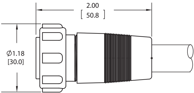
13XXX-XXG CUSTOM CABLE CONNECTOR STRAIGHT OVERMOLDED
