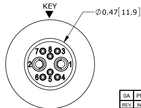
WIRING END ASSY: W7A82-8PG-300 SHOWN
