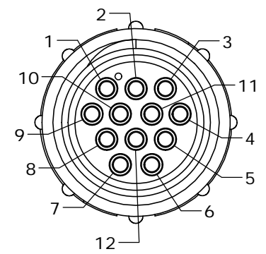
WIRE VIEW
