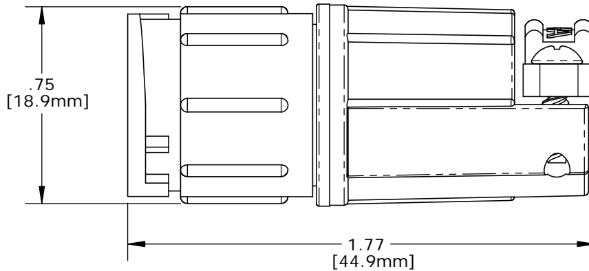
ASSEMBLED VIEW
