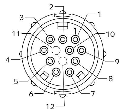
MATING FACE W5280-10PG-5XX
