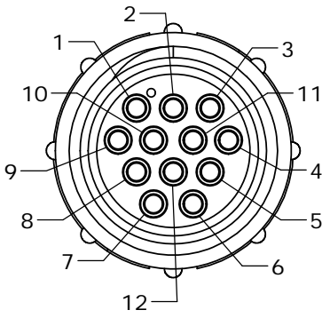
WIRE VIEW
