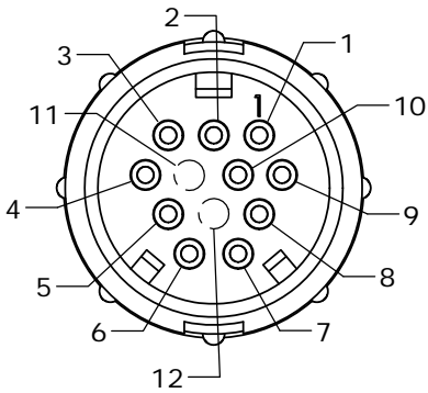
FACE VIEW W5280-10PG-3XX
