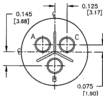
SIZE: 16-10 3-#12 CONTACTS
