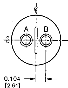
SIZE: 12S-3 2-#16 CONTACTS
