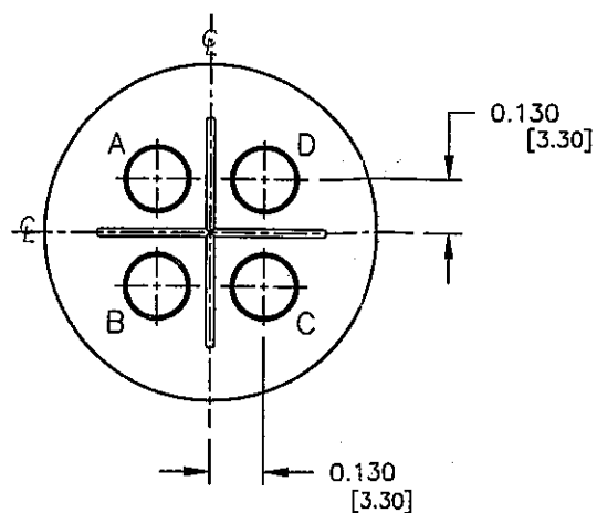
SIZE: 18-10 4-#12 CONTACTS
