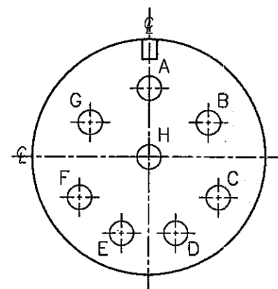
SIZE: 20-7 8-#16 CONTACTS
