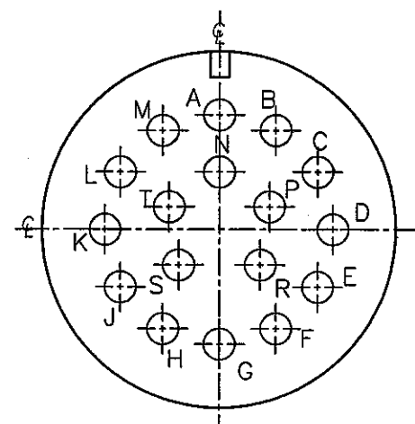
SIZE: 20-29 17-#16 CONTACTS
