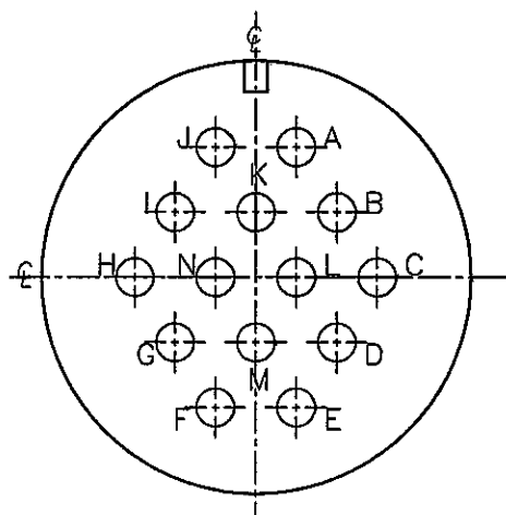
SIZE: 20-27 14-#16 CONTACTS
