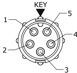
FACE VIEW 8380-5PG-5XX
