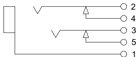
SCHEMATIC
