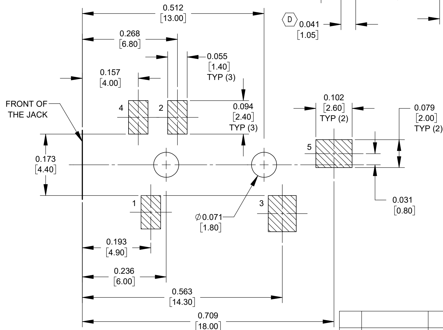
PCB LAYOUT COMPONENT SIDE TOLERANCE: \pm 0.002 [ \pm 0.05 ]
