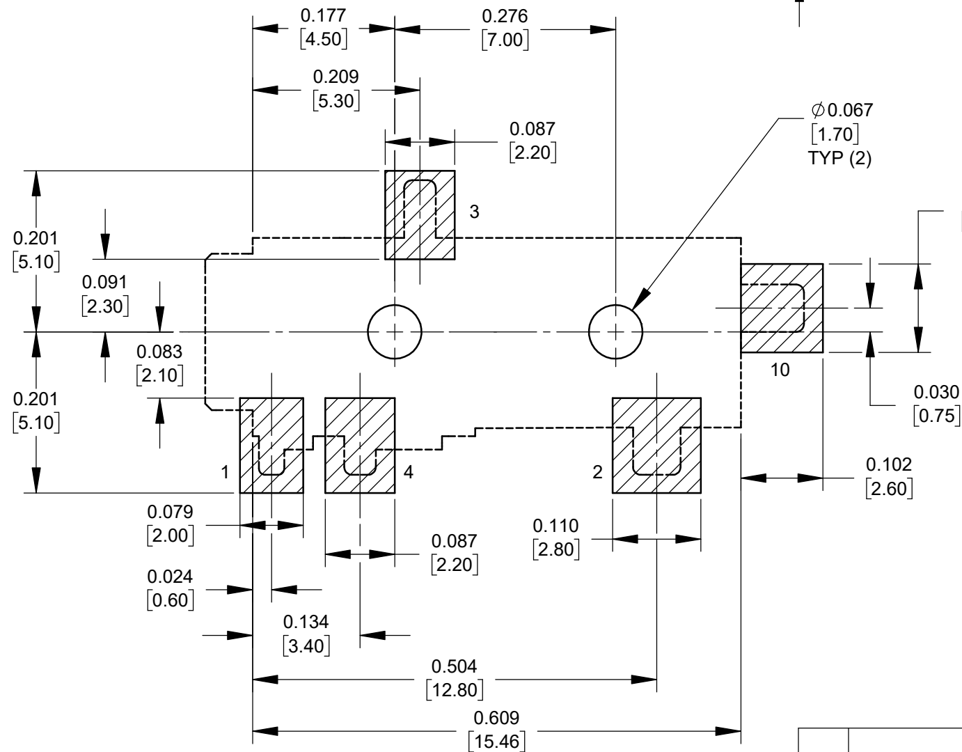
PCB LAYOUT COMPONENT SIDE
