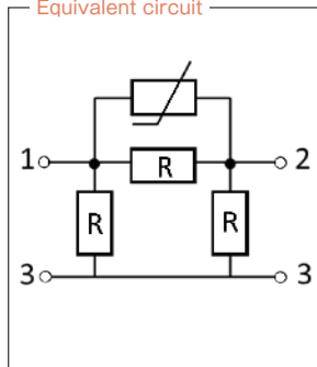
Equivalent circuit
