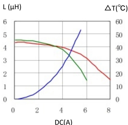
5. CDRH8D43RT125NP-4R3NC
