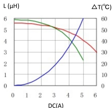
6. CDRH8D43RT125NP-5R6NC
