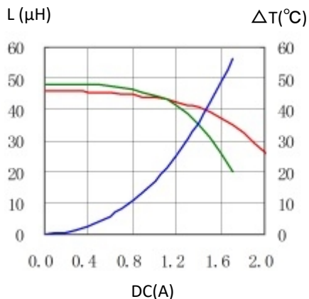
13. CDRH8D43RT125NP-470MC
