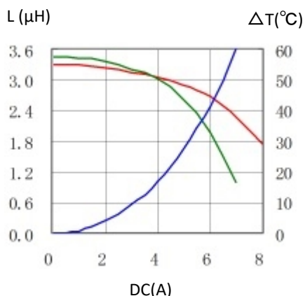
4. CDRH8D43RT125NP-3R3NC
