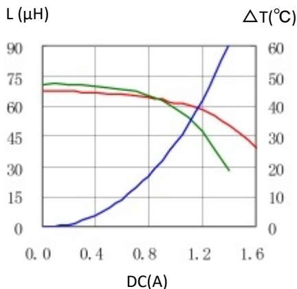
14. CDRH8D43RT125NP-680MC
