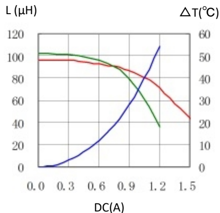
15. CDRH8D43RT125NP-101MC
