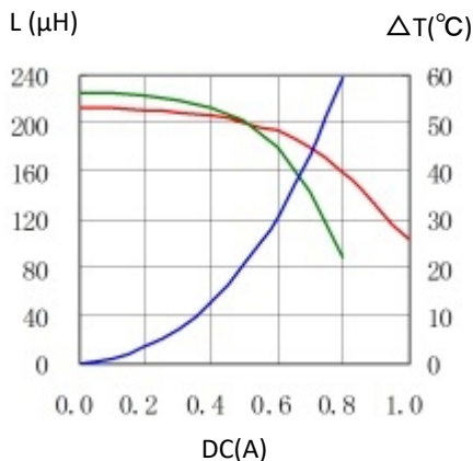
17. CDRH8D43RT125NP-221MC
