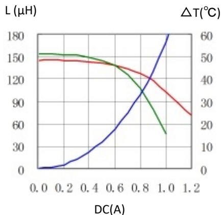
16. CDRH8D43RT125NP-151MC
