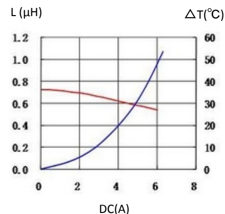
6. 0320CDMCCDS-R82MC
