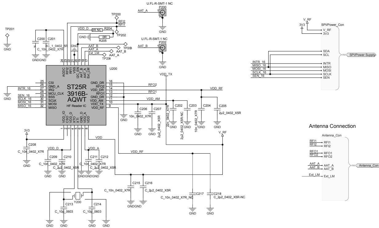
Figure 2. X-NUCLEO-NFC08A1 circuit schematic (2 of 3)
