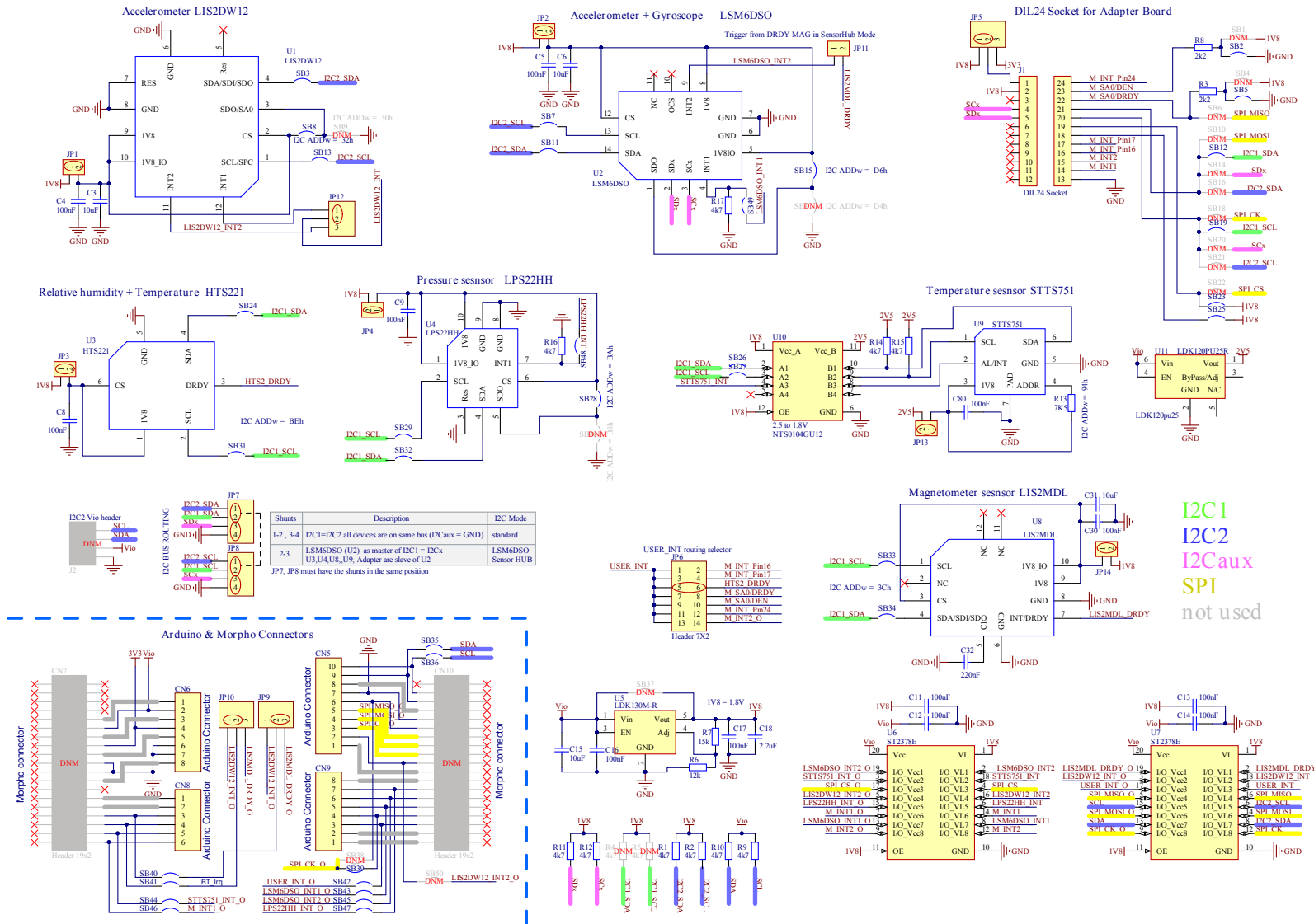
Figure 1. X-NUCLEO-IKS01A3 board schematics
